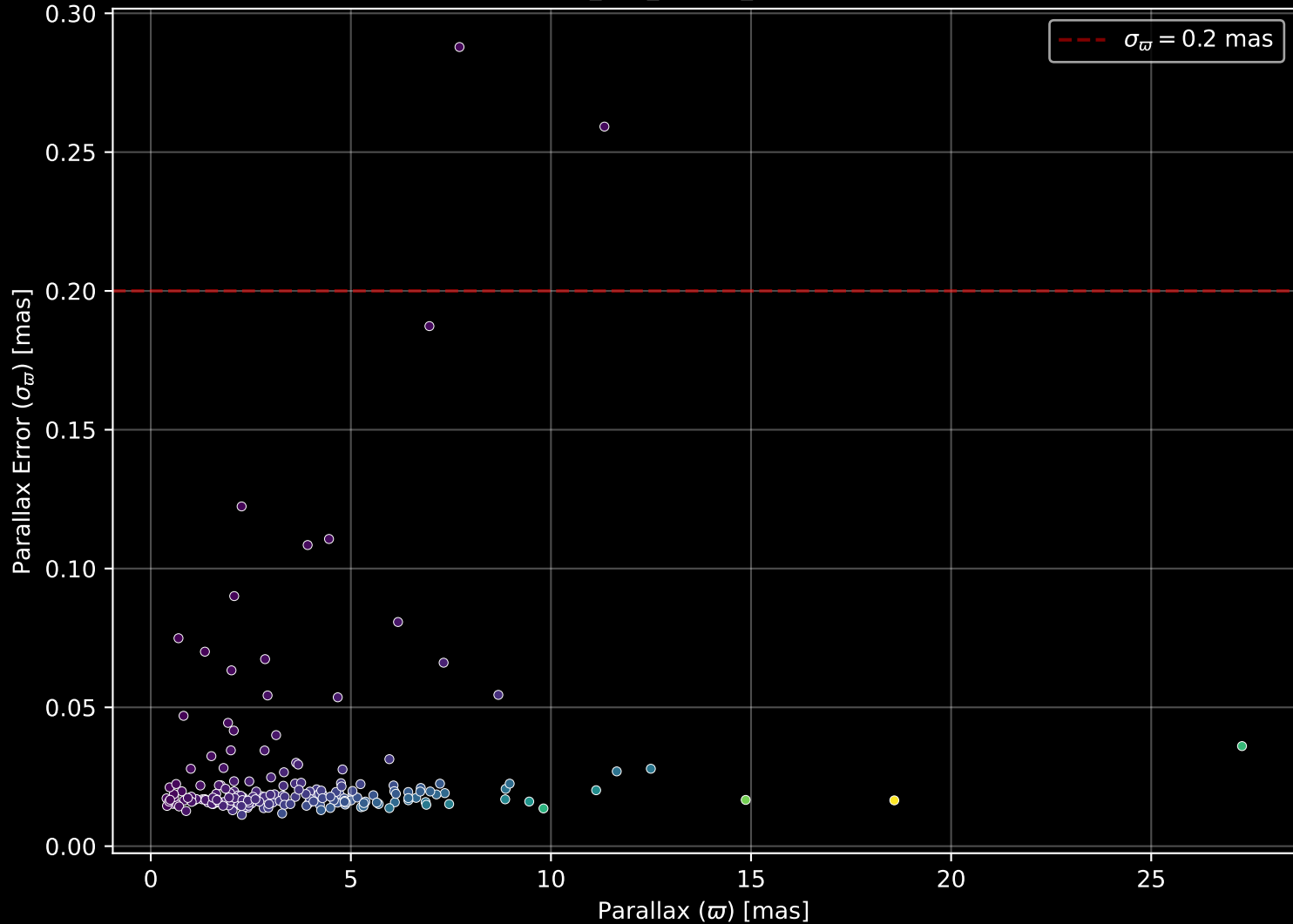
APOGEE DR17 Field: [K2_C12_082-54_btx] Parallax Quality (n= 194)
