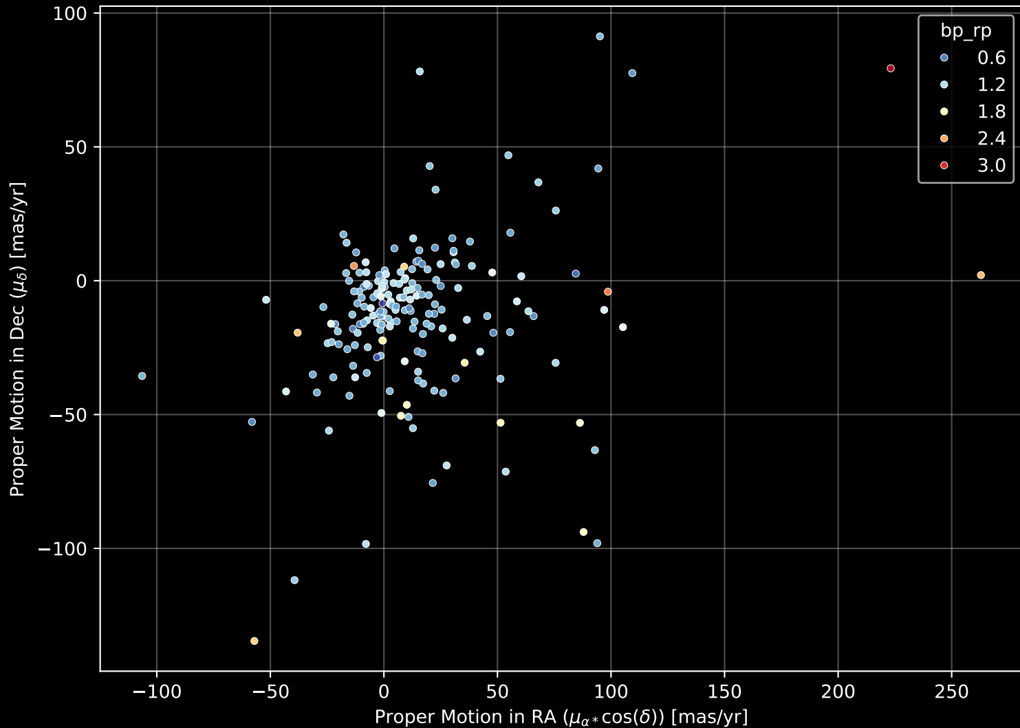
APOGEE DR17 Field: [K2_C12_082-54_btx] Proper Motion Diagram (n= 194)
