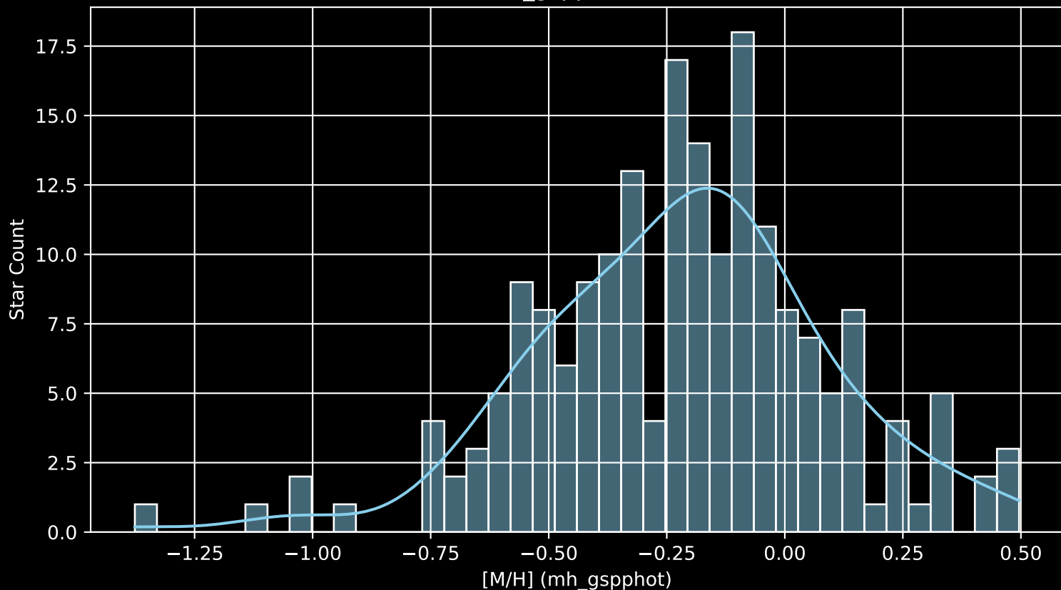
APOGEE DR17 Field: [K2_C12_082-54_btx [M/H] (mh_gspphot) (n= 192)
