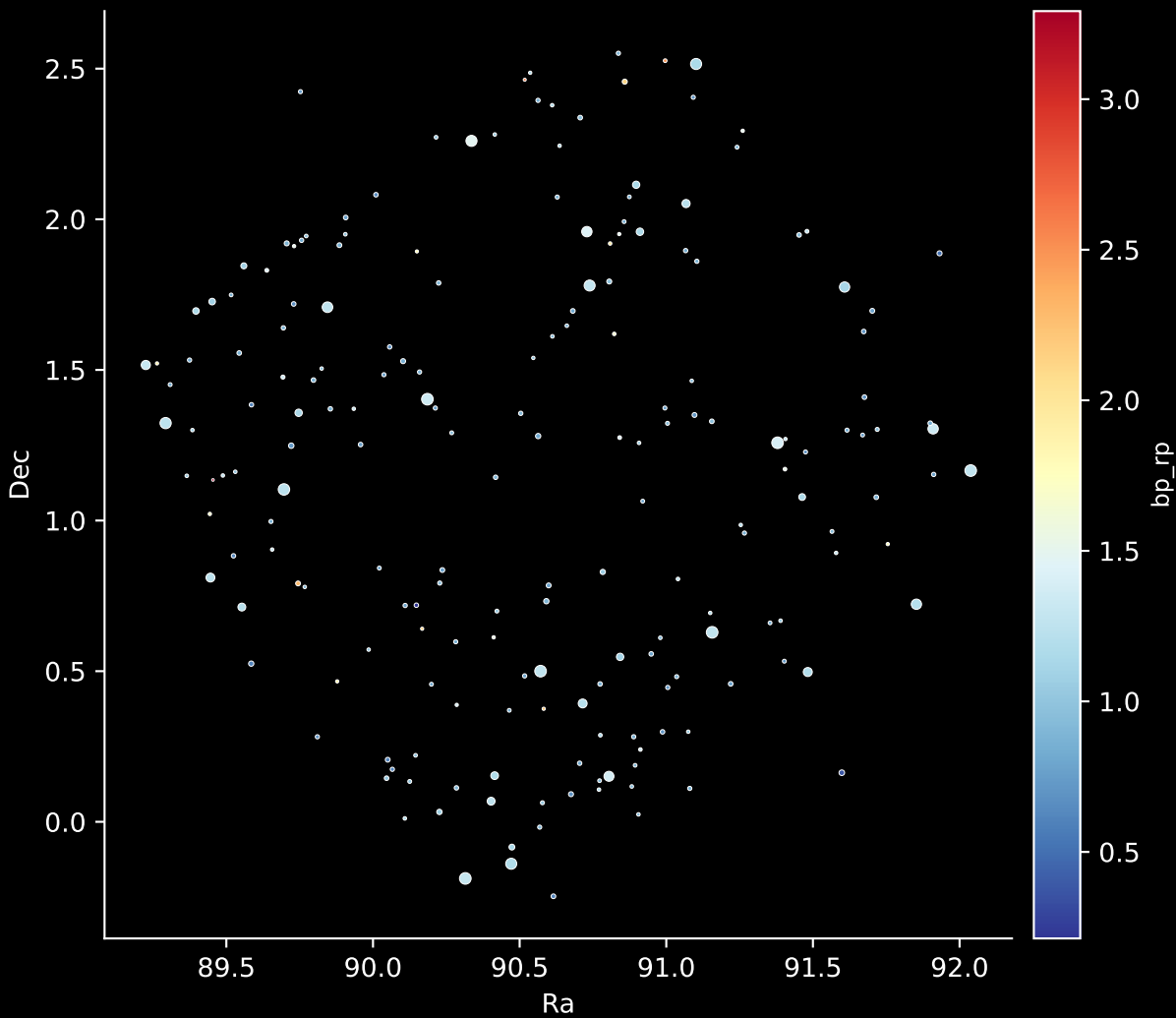
APOGEE DR17 Field: [K2_C12_082-54_btx] Stars: 194
