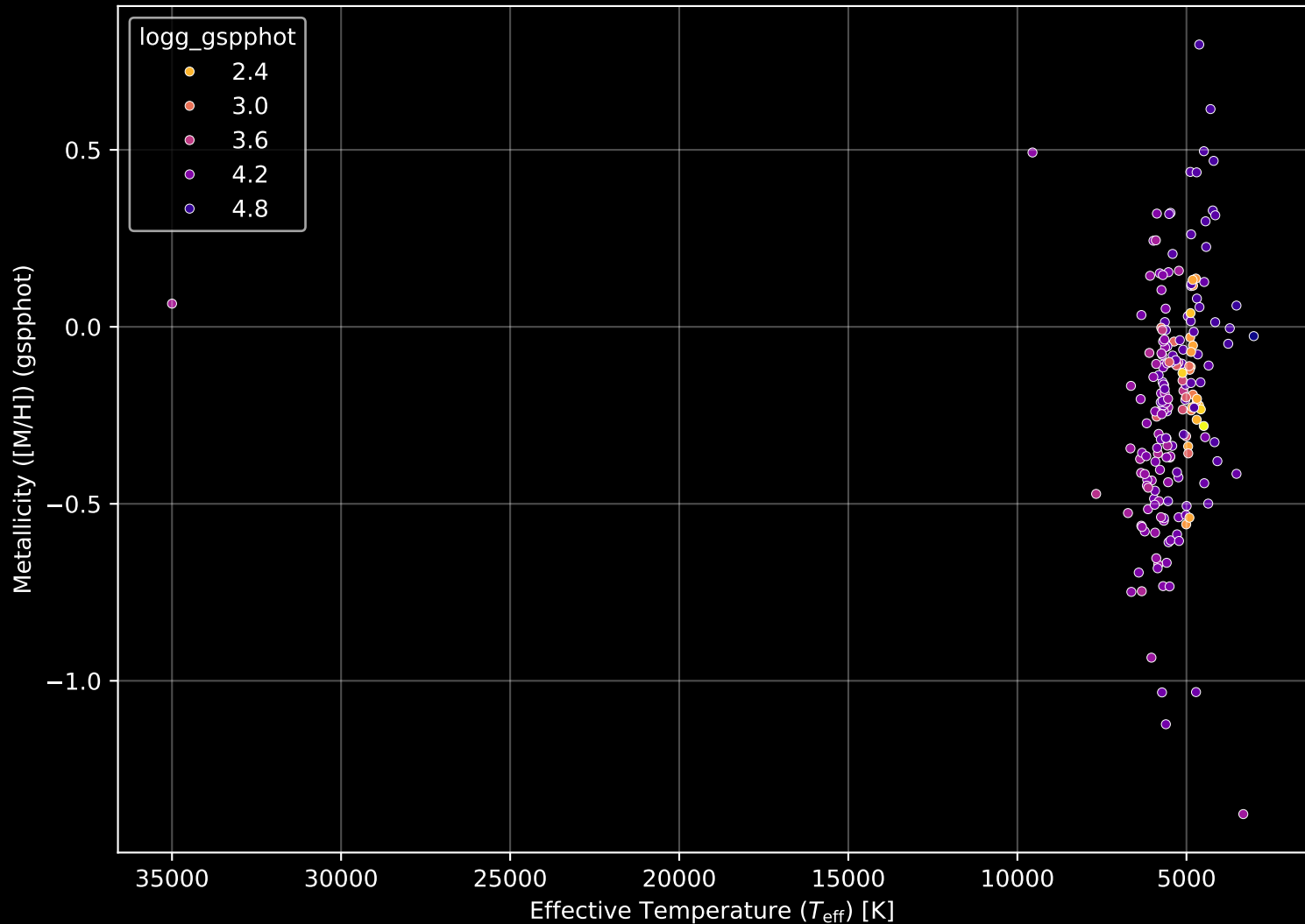
APOGEE DR17 Field: [K2_C12_082-54_btx] Stellar Population Parameters (n= 194)
