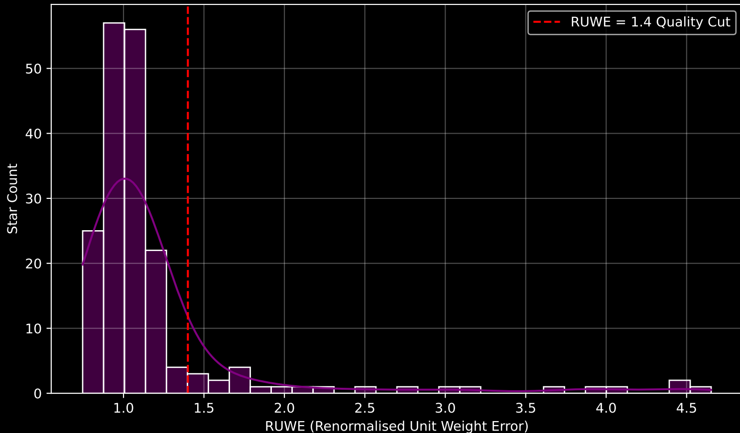
GAPOGEE DR17 Field [K2_C12_082-54_btx] RUWE Distribution (n= 187)
