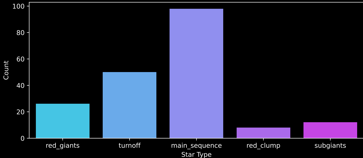
APOGEE DR17 Field: [K2_C12_082-54_btx] Count plot of Star Type
